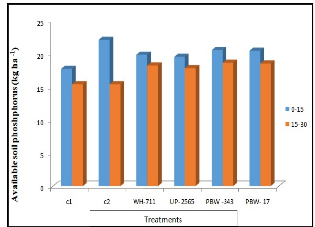
Fig 5. Effect of open farming and Eucalyptus based agroforestry systems on available soil phosphorus kg ha -1 and their interaction at different profile depths 0 -15 and 15 – 30 cm
