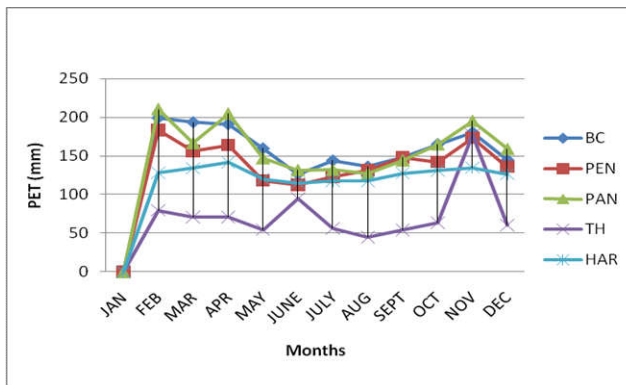
Fig. 5: PET for Muhuru Bay (1976-1986)
