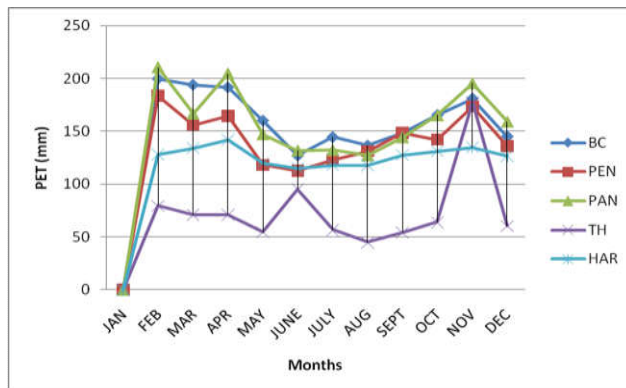
Fig. 6: PET for Kadenge (1976-1986)
