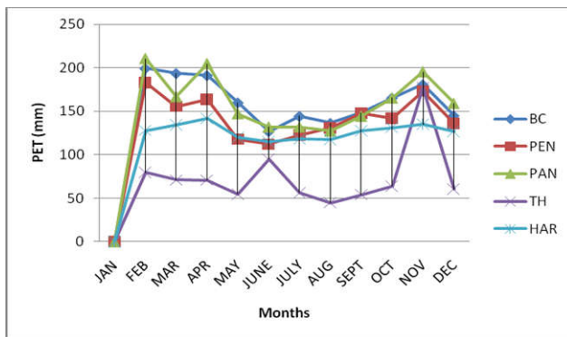
Fig. 4: PET for Rusinga Island (1976-1986)
