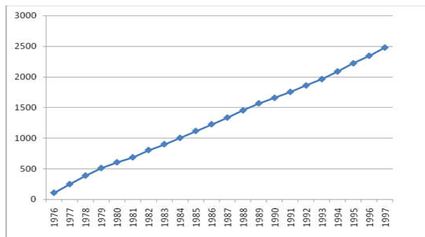
Figure 3: Mass curve using data from Kisumu Airport meteorological station
