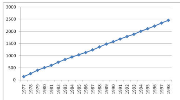
Figure 2: Mass curve using data from Kibos Cotton Research Station
