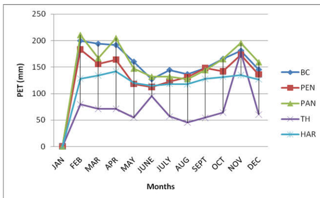
Fig. 7: PET for Kisumu Airport (1976-1986)
