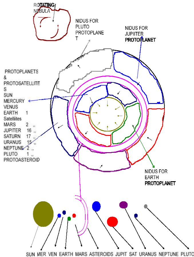
Figure 12. Origin of solar system
