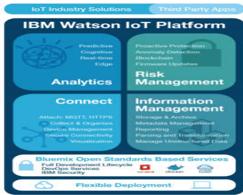
Figure 3. IBM Watson Platform
