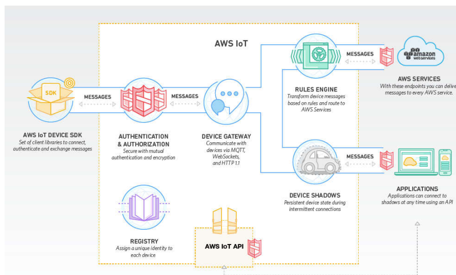
Figure 6. Amazon Web Services Infrastructure Design
