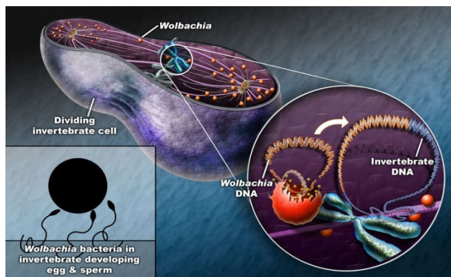
Fig.1. Wolbachia enters the host cell, and then Wolbachia DNA is incorporated into DNA of host cell
